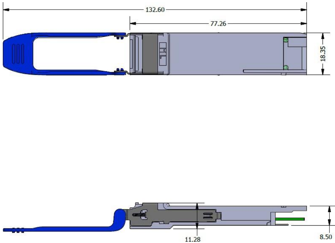
Figure 10: Mechanical Dimensions
