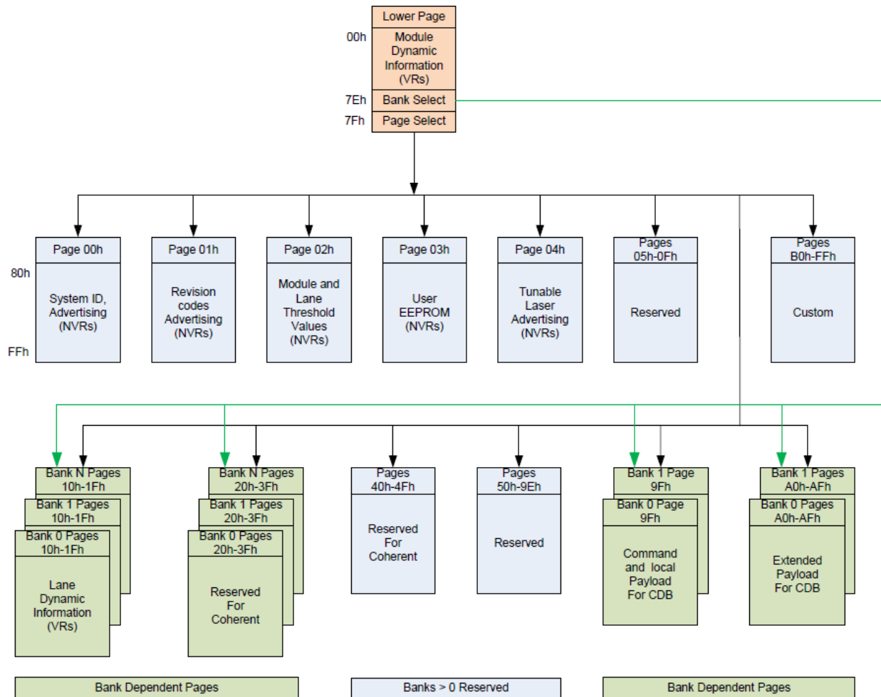
Figure 3: QSPF-DD Memory Map
