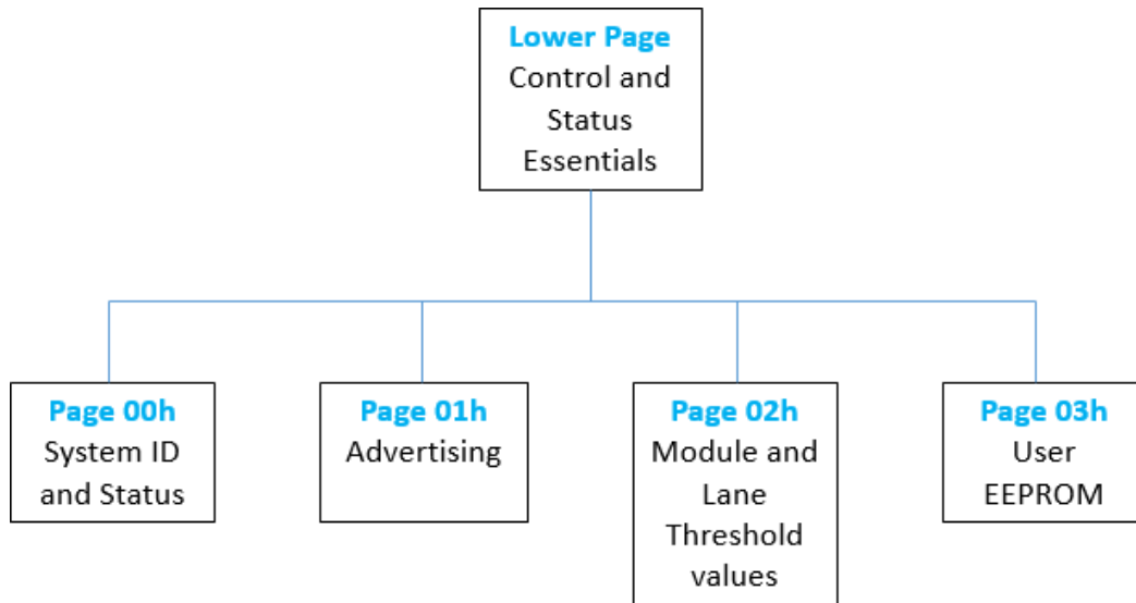
Figure 4: Implemented Memory Map
