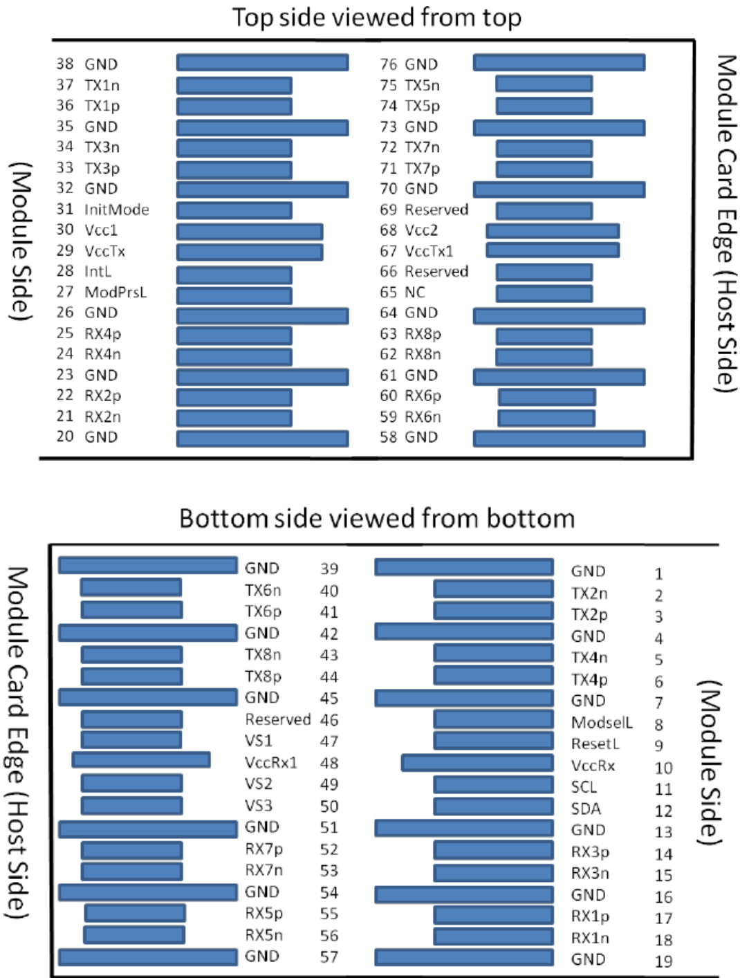
Figure 9: QSFP-DD Module Pad Layout
