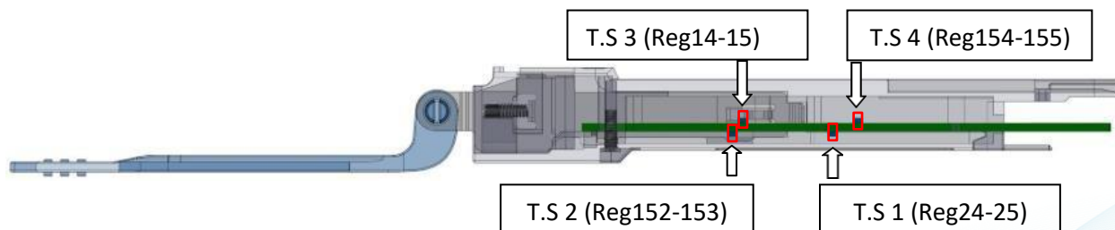
Figure 5: temperature sensor location
